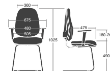
TPGC/1D: Overall Dimensions: 675w x 640d x 1025h
