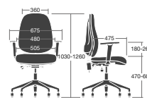
TPG/1D: Overall Dimensions: 690w x 690d x 1260h
