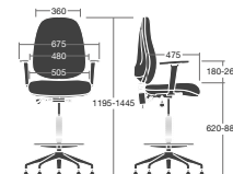
TPGD/1D: Overall Dimensions: 690w x 690d x 1445h
