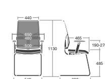
MIXC/4D: Overall Dimensions: 690w x 690d x 1130h
