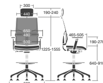
MIXD/4D/UR: Overall Dimensions: 690w x 690d x 1795h
