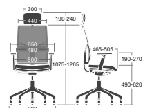
MIX/4D/UR: Overall Dimensions: 690w x 690d x 1505h
