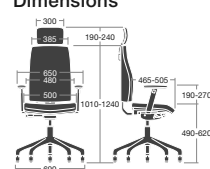
MAT/4D/UH: Overall Dimensions: 690w x 690d x 1480h
