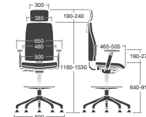
MATD/4D/UH: Overall Dimensions: 690w x 690d x 1770h
