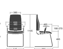
MATC/4D: Overall Dimensions: 600w x 680d x 1105h
